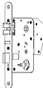
EURO Auto Deadbolt upgrade kit ( DAVINCI ), (available from Dec. 03)
